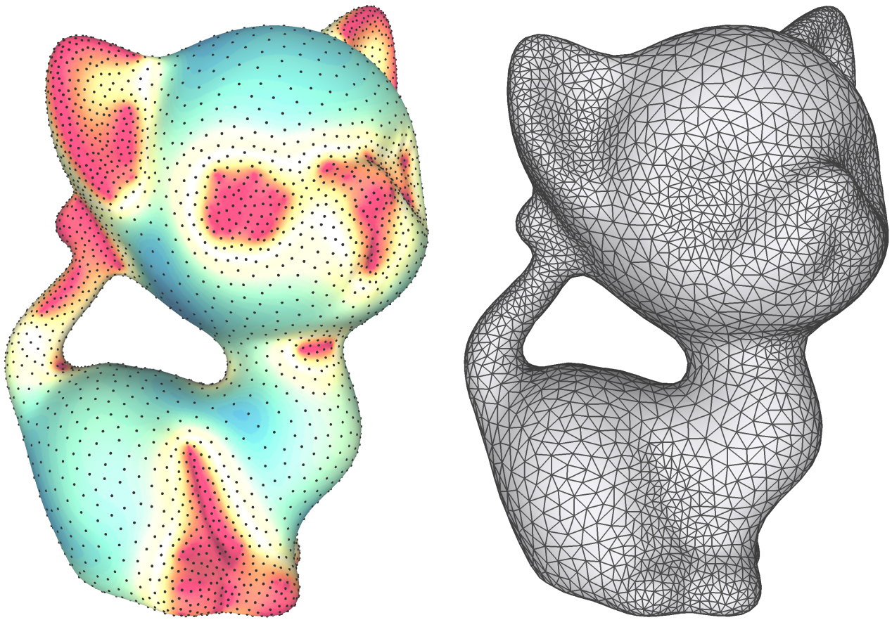
Figure 9: Kitten 3D model with 4k generated points (left) and remeshing result (right).
