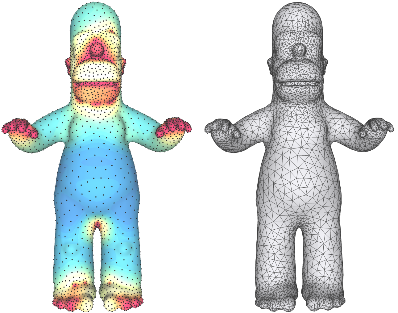
Figure 10: Homer 3D model with 3.5k generated points (left) and remeshing result (right).
