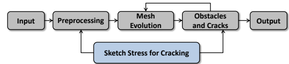
Figure 3: System Overview. A polygonal model is converted to a tetrahedral mesh during preprocessing. The mesh is evolved by using our developmental model and, at the same time, is covered by cracks and checked for collisions in the surrounding environment. The user can control the definition of the cracks and the growth function.
