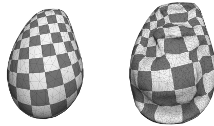
Figure 9: Texture coordinates are preserved after DSC propagation and numerous remeshing operations.
